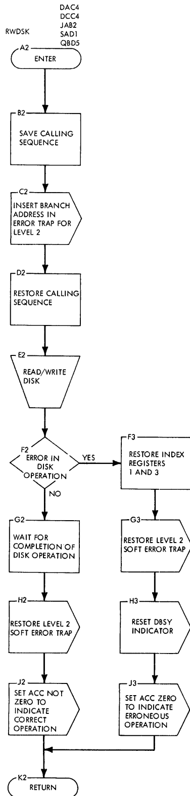
Chart RB. (RWDSK) Read/Write Disk
