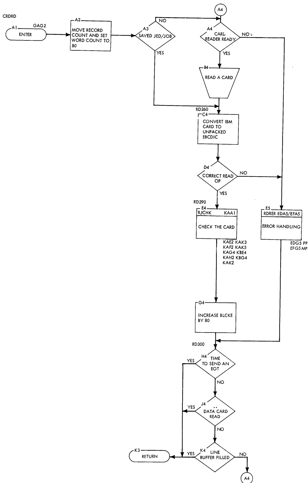
Chart HA. (CRDRD) Card Read Input Routine
