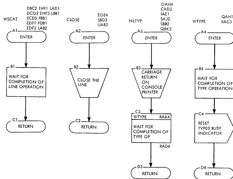
Chart RA. (RJL0n) Miscellaneous Subroutines
