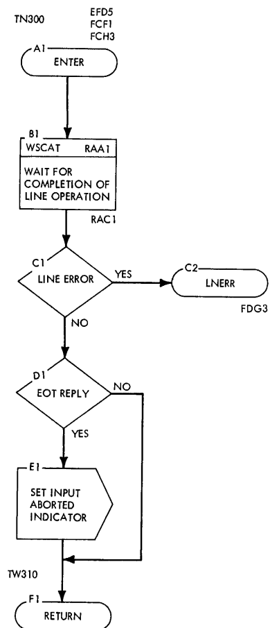
Chart FD. (RJTWM) Write Multipoint Subroutines
