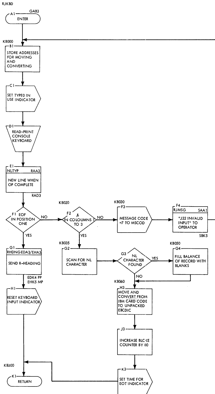
Chart IA. (RJKBD) Console Keyboard Input
