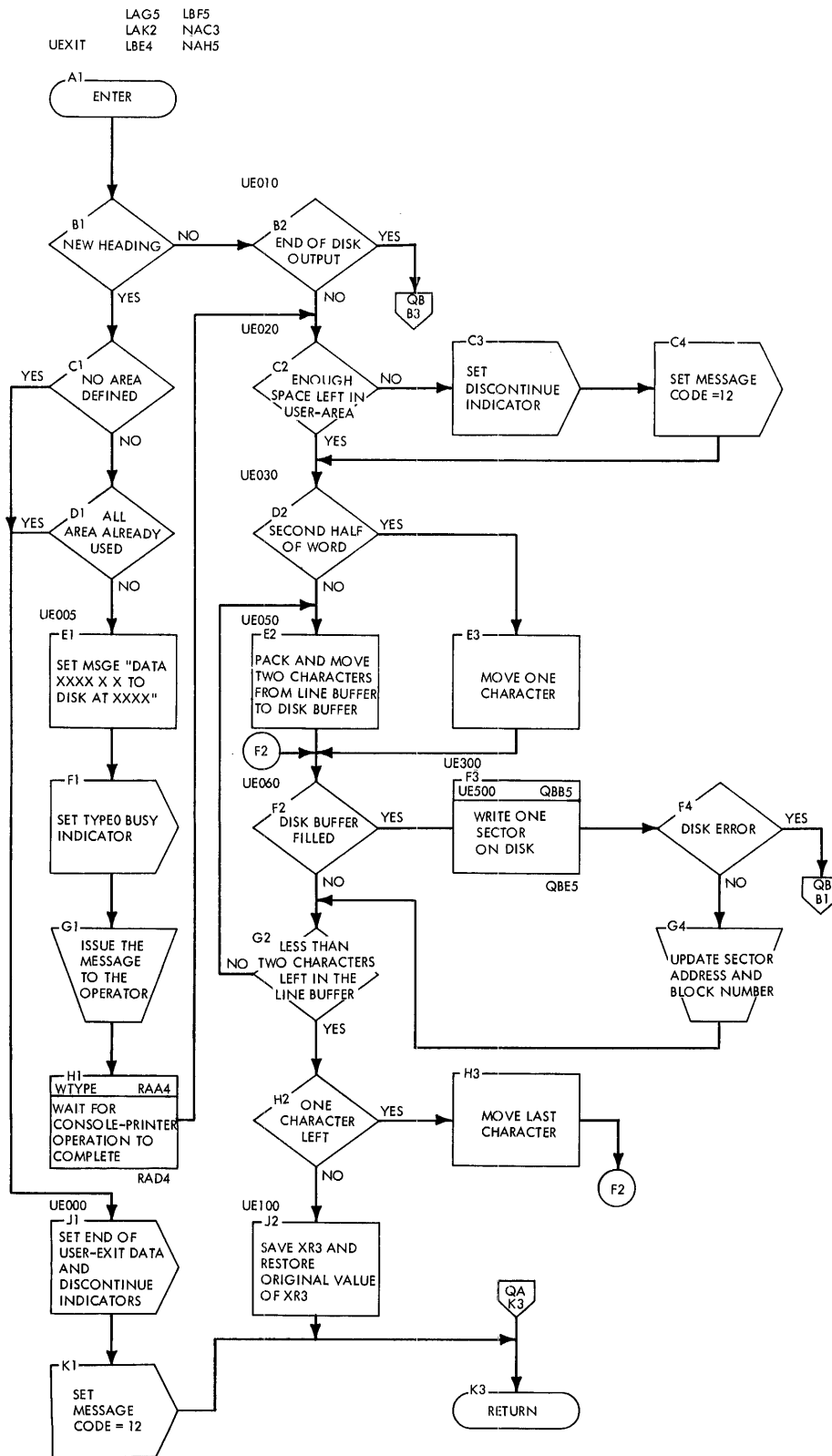
Chart QA. (UEXIT) User-exit Routine
