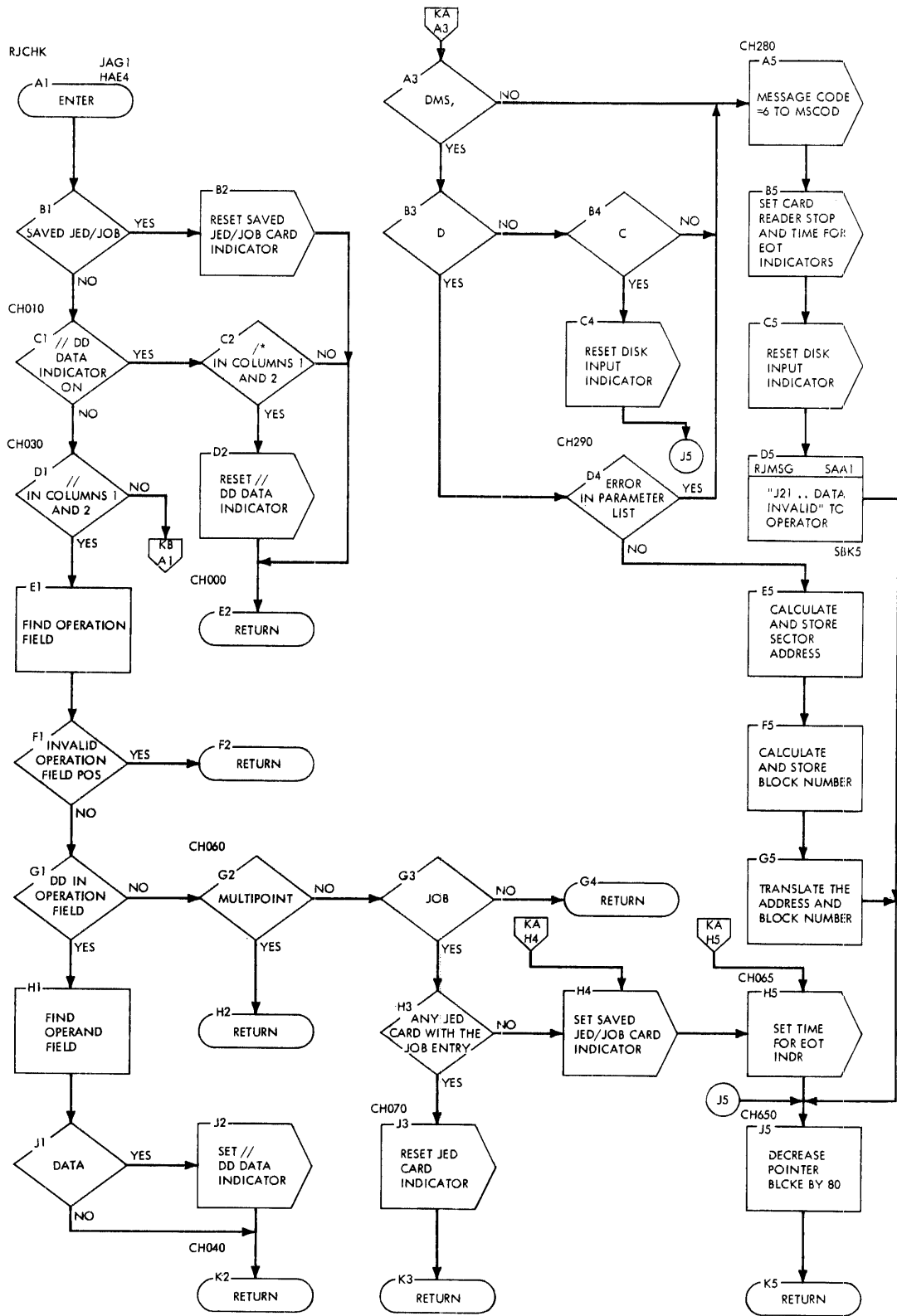
Chart KA. (RJCHK) Card Check Routine
