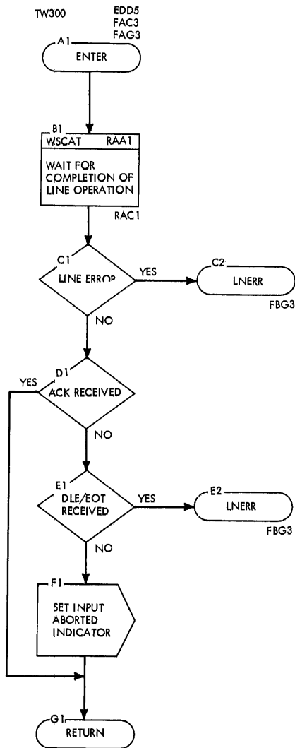
Chart FB. (RJTWP) Write Point-to-Point Subroutines
